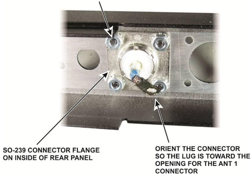
Figure 20. Installing the XMTR SO-239 Connector in the Rear Panel.
