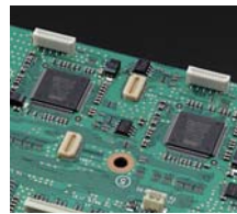
Transmit/ Receiver DSP (left) and Receiver DSP (right) ADSP-21489 by Analog Devices 32-bit floating point DSP 2400 MFLOPS 393 MHz clock speed
